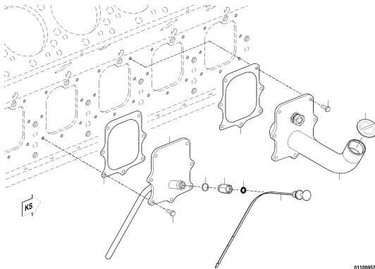
INSPECT PORT COVER FOR OIL DIPSTICK XS528010.00008
