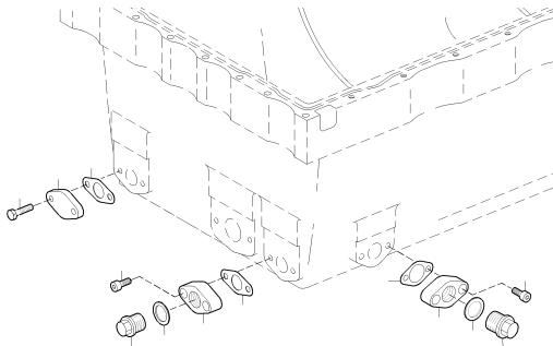
SEAL ELEM. FOR OIL PAN X00030756
