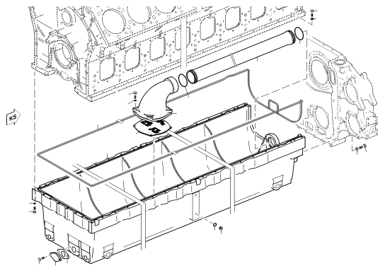
OIL PAN 010.00170
